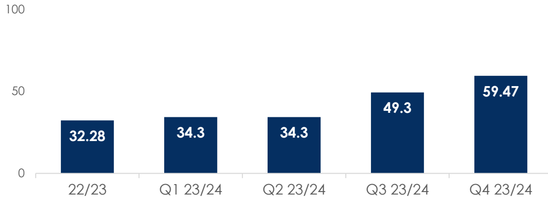
% of Council housing meeting Scottish Housing Quality Standards (SHQS) (cumulative)
